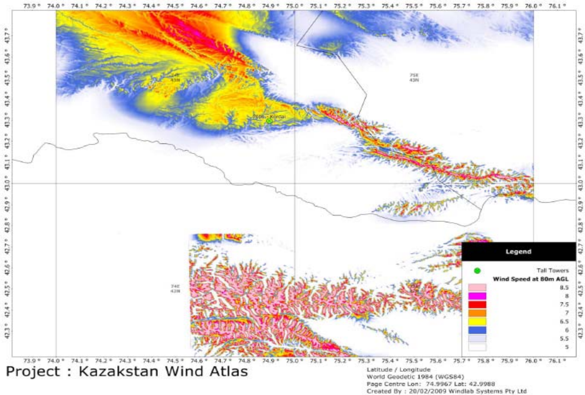
Figure 2. Wind map of the area around Kordai of Zhambylskaya oblast at a height of 80 m above ground level and a resolution of 100 m.
