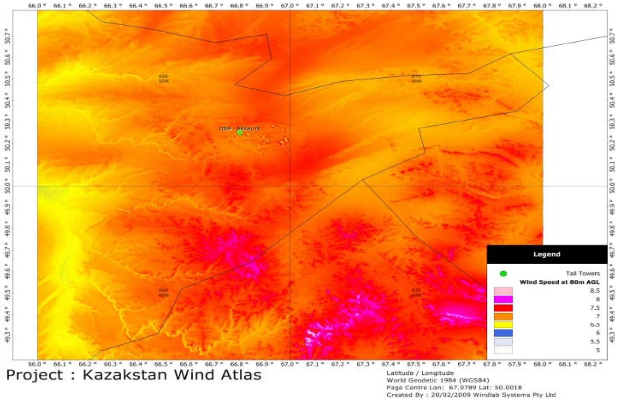
Figure 2. Wind map of the area around Arkalyk of Kostanaiskaya oblast at a height of 80 m above ground level and a resolution of 100 m.
