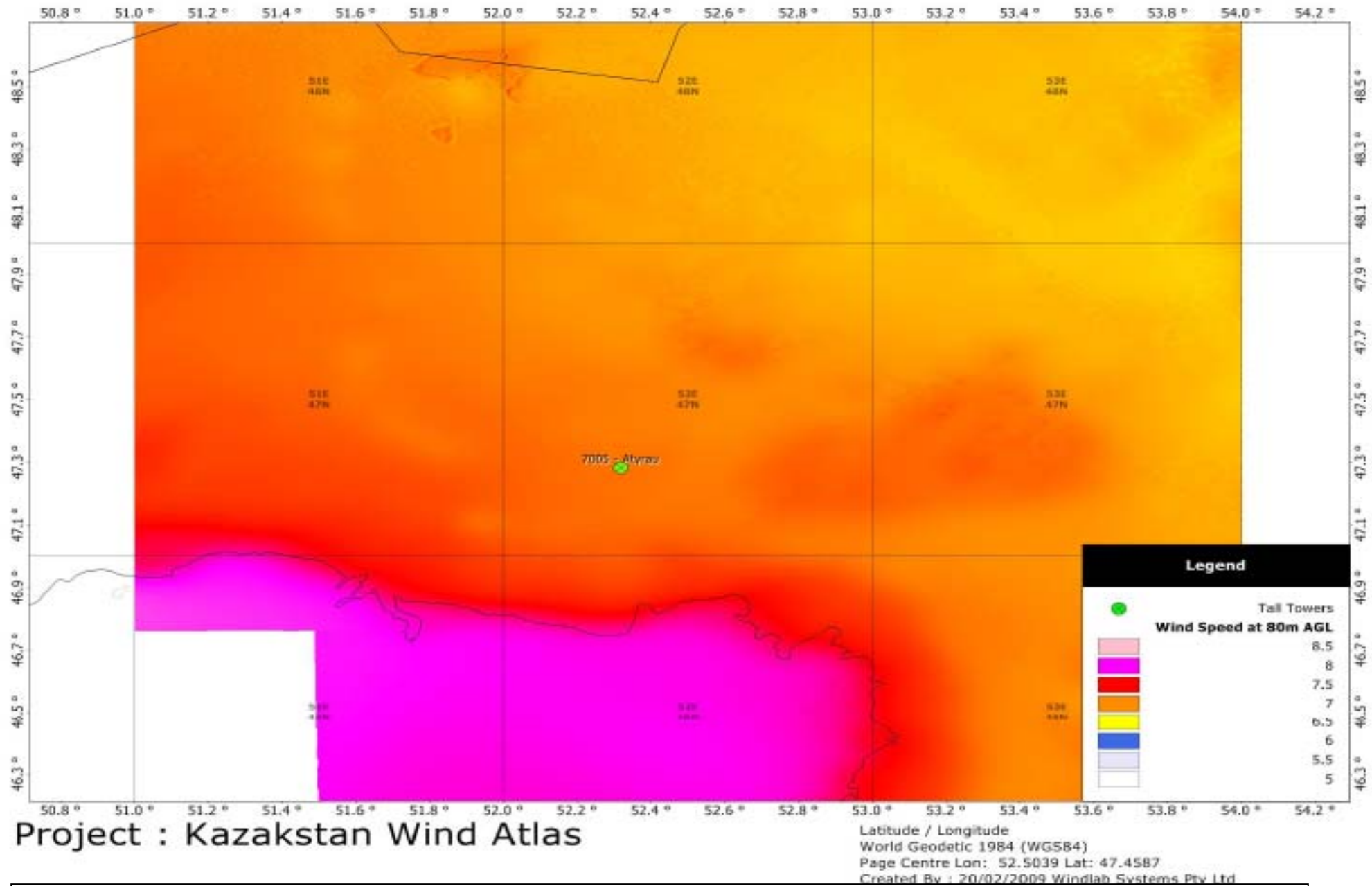
Figure 2. Wind map of the area around Atyrau of Atyrauskaya oblast at a height of 80 m above ground level and a resolution of 100 m
