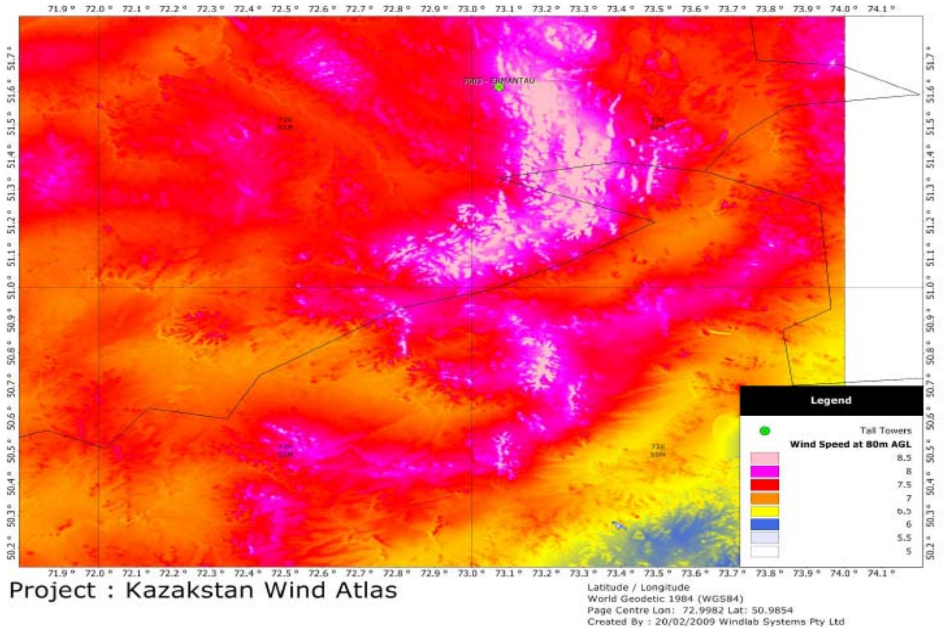
Figure 3. Wind map of the area around Ereymentau of Akmolinskaya oblast at a height of 80 m above ground level and a resolution of 100 m.
